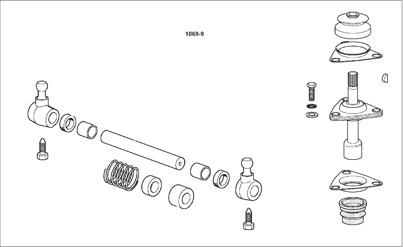
Fig. 5 - Internal shuttle control.
