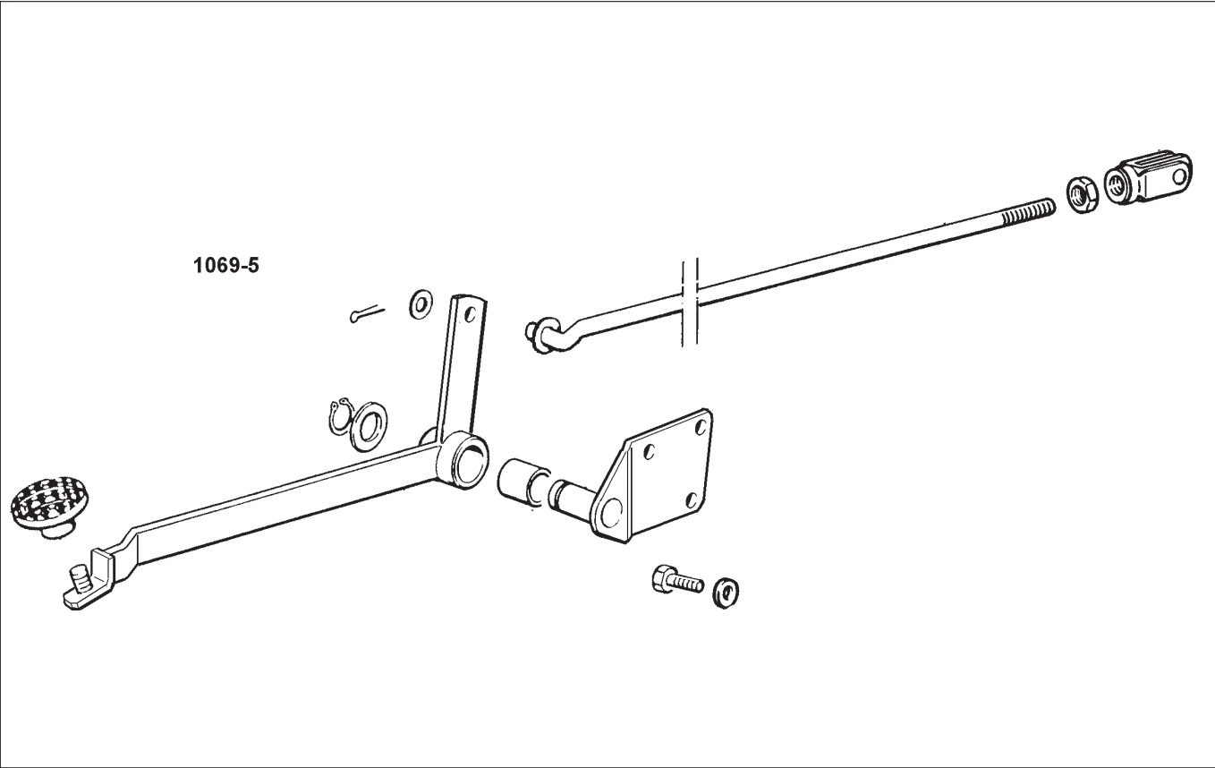
Fig. 6 - Differential lock control.
