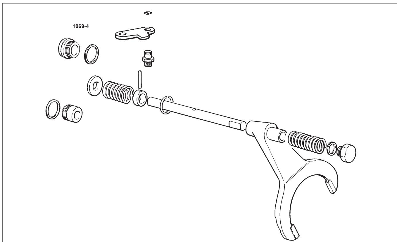
Fig. 7 - Internal differential lock control.
