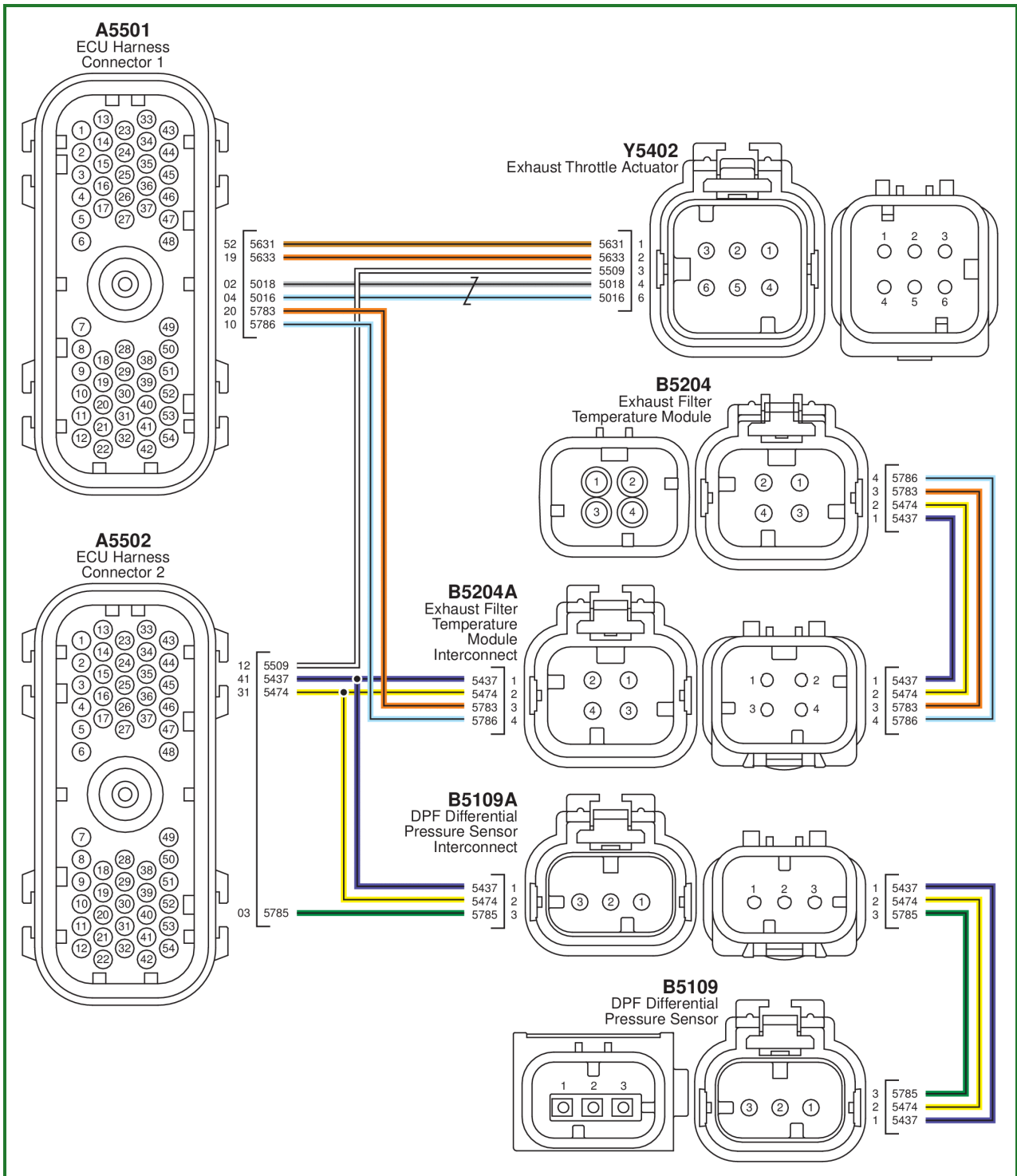
RG24384-UN: 2.9 L Wiring Diagram 4
