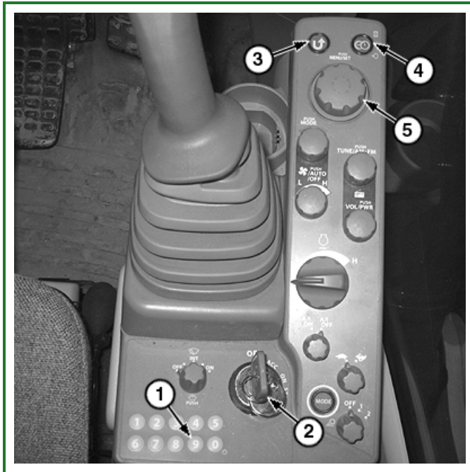
TX1086439A-UN: Right Console Panel
