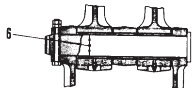
Section J—J
