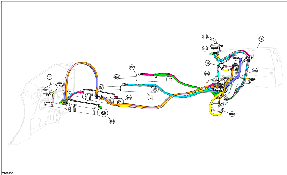
T202636-UN: Main Hydraulic Component Location
