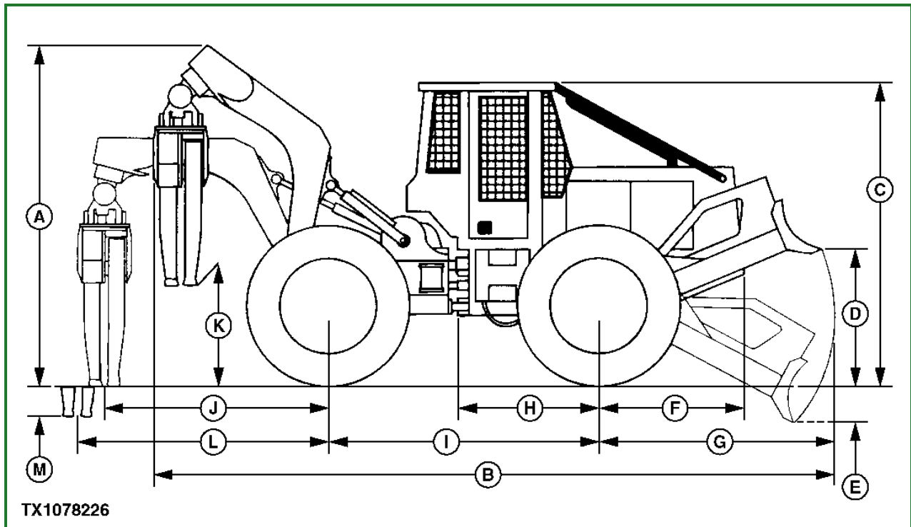
TX1078226-UN: Grapple Skidder Dimensions—Side View
