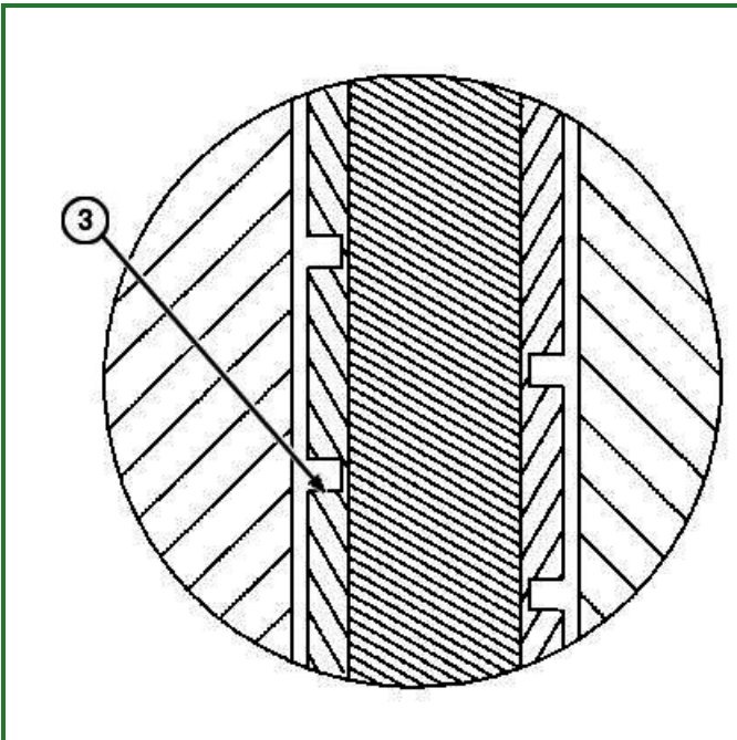
TX1015685A-UN: Brake Lining Oil Grooves
