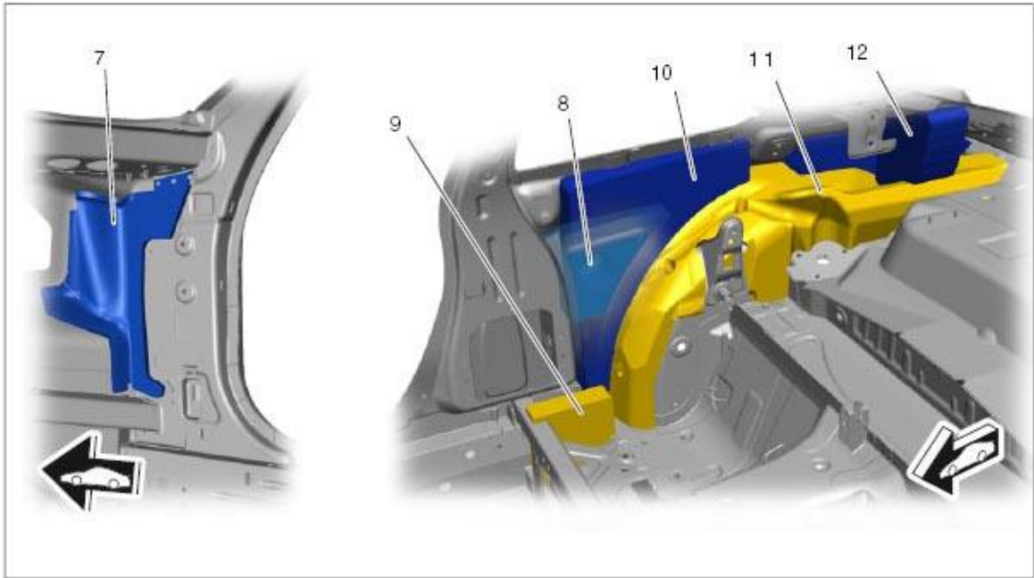
Fig. 2: Overview Of Sound Absorbers For Passenger Compartment - Right Courtesy of PORSCHE CARS NORTH AMERICA, INC.
