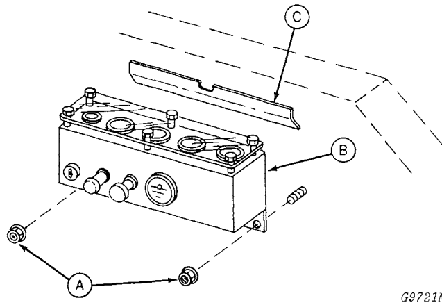
A—Lock Nuts B—Instrument Panel C—Support Ledge
