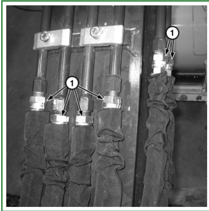
TX1134531A-UN: Boom Hydraulic Lines
