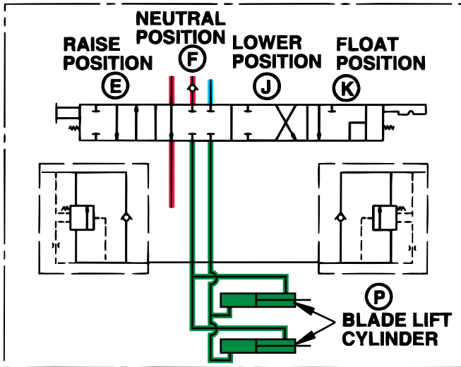
(Q) BLADE LIFT SECTION - NEUTRAL
