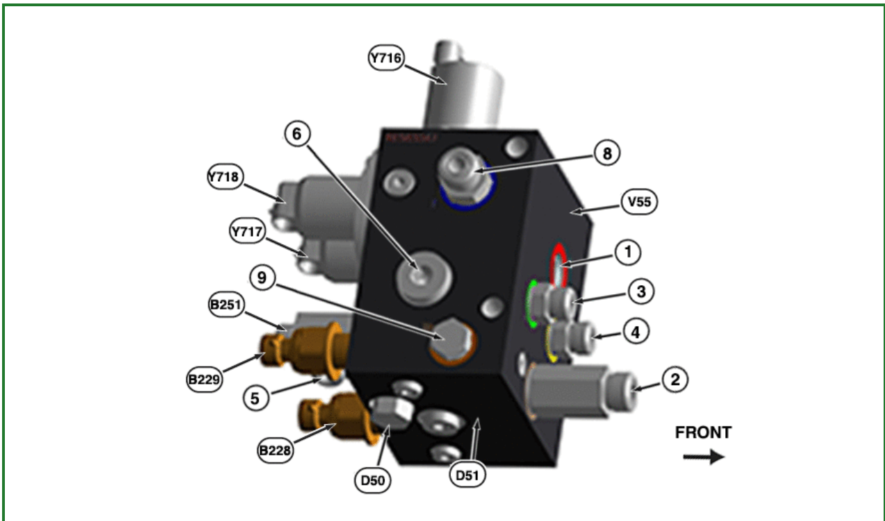
RXA0164705-UN: Secondary Brake and Steering Control Valve ( Right Hand side)
