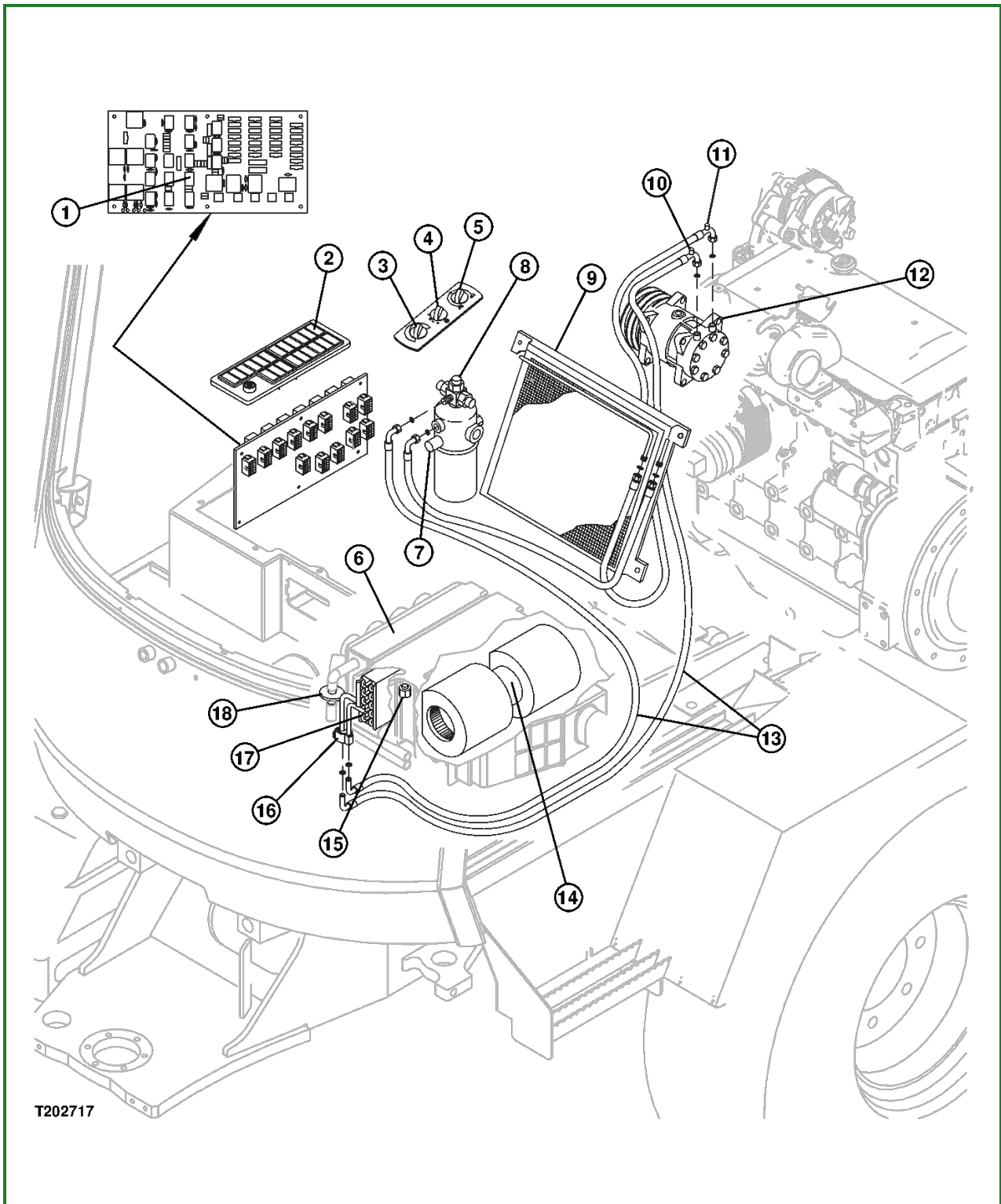
T202717-UN: Air Conditioner and Heater Component Location
