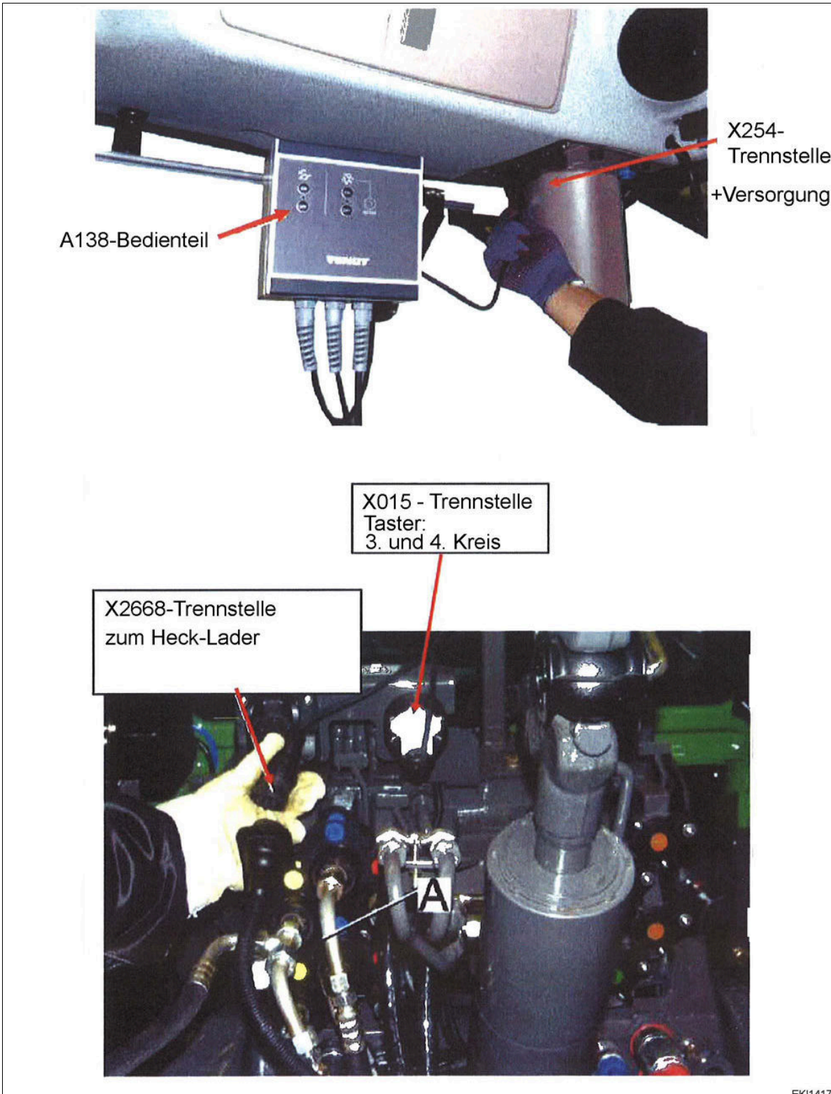
Fig. 3. Connect A138 control panel in the tractor
