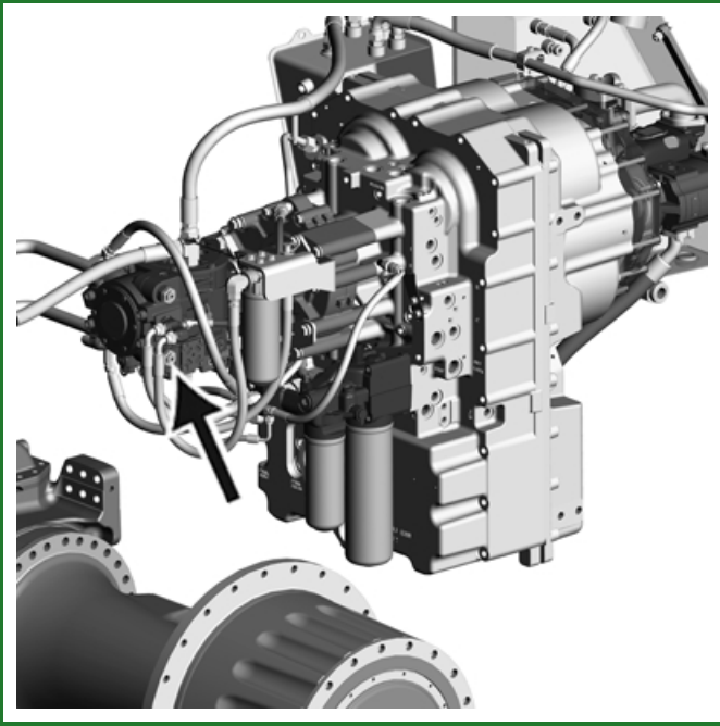
RXA0138495-UN: V66 Multifunction Valve
