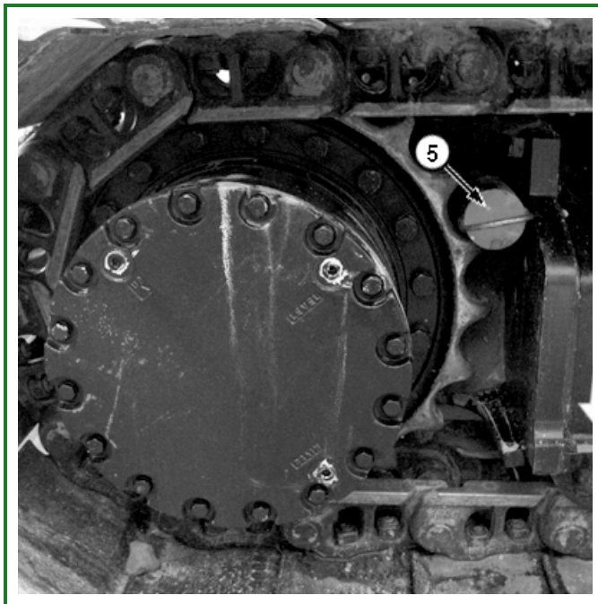
TX1104361A-UN: Travel Motor Stalled Using Pin
