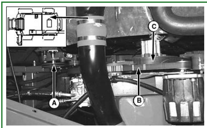
H77787-UN: Radiator Fan and Rotary Screen Drive - 6125 Engine
