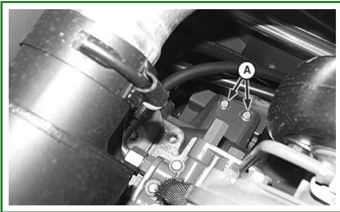
H55531-UN: Front Main Gearcase Mounting Hardware
