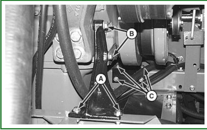
H70287-UN: Front Engine Mount Engine Type B
