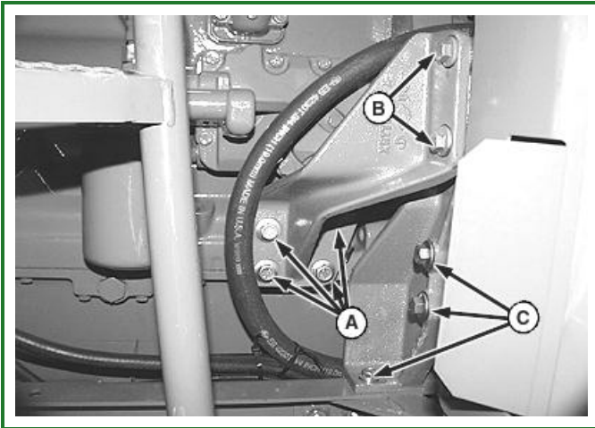
H70289-UN: Front Engine Mounts Engine Type A
