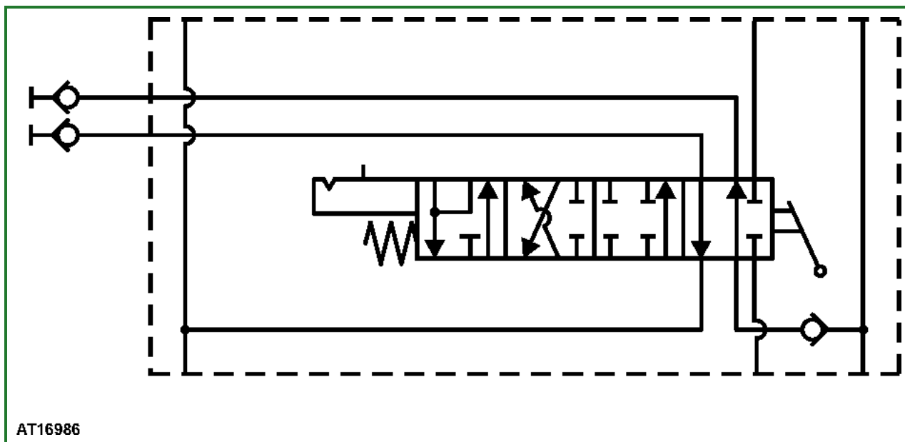
AT16986-UN: SCV operation (double-acting) - position 1
