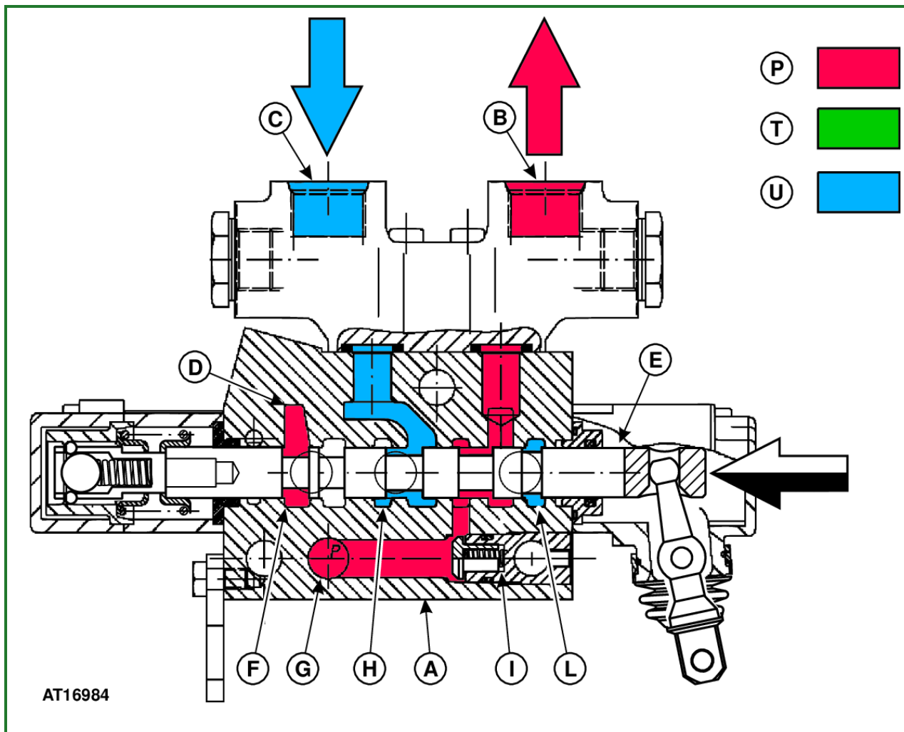
AT16984-UN: SCV operation (double-acting) - position 1
